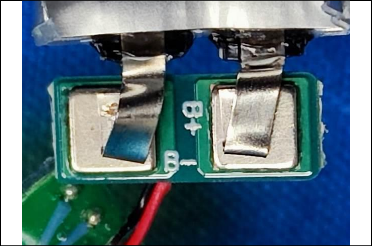
Battery PCB view
