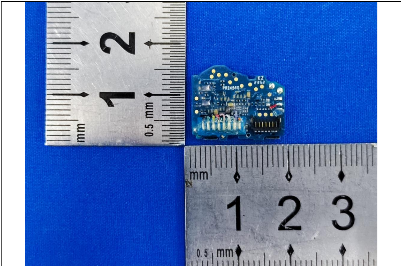
PCB view
