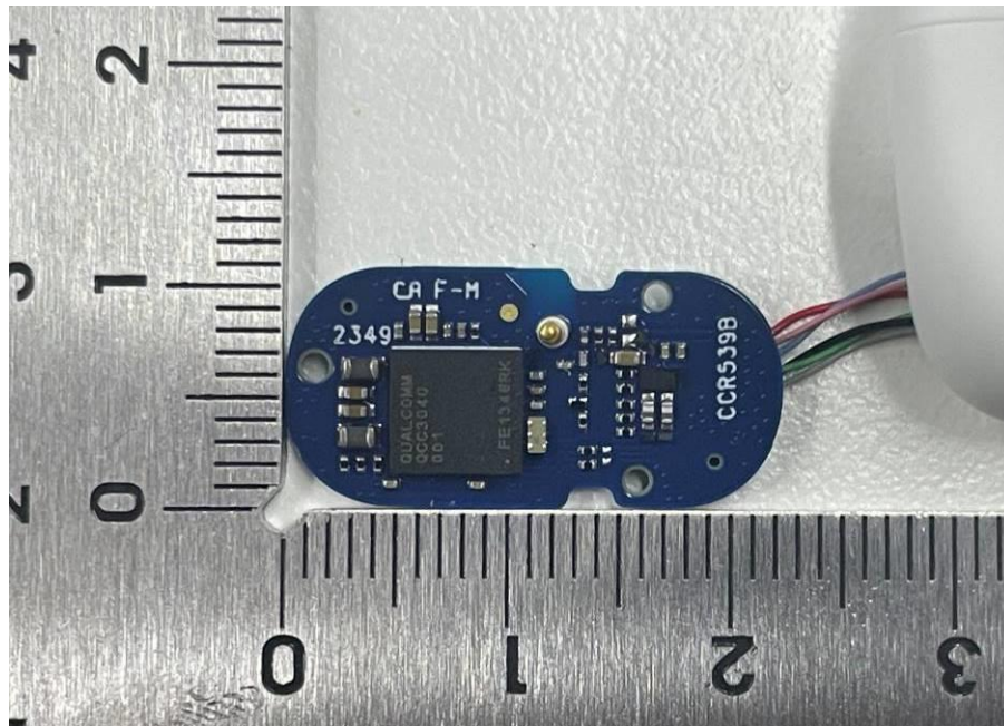
Figure 16: PCB view 2 of right earbud
