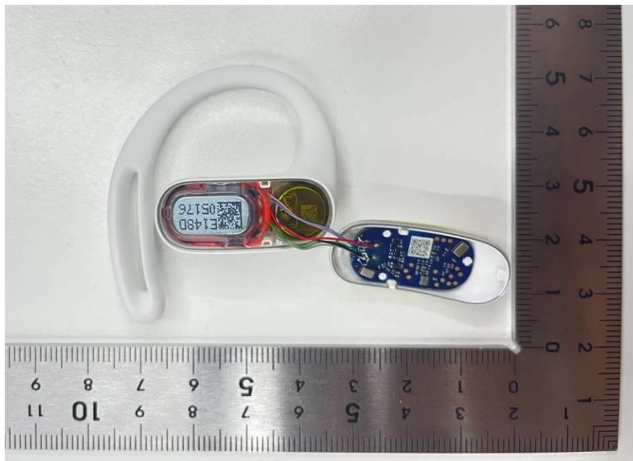
Figure 14: Internal view of right earbuds
