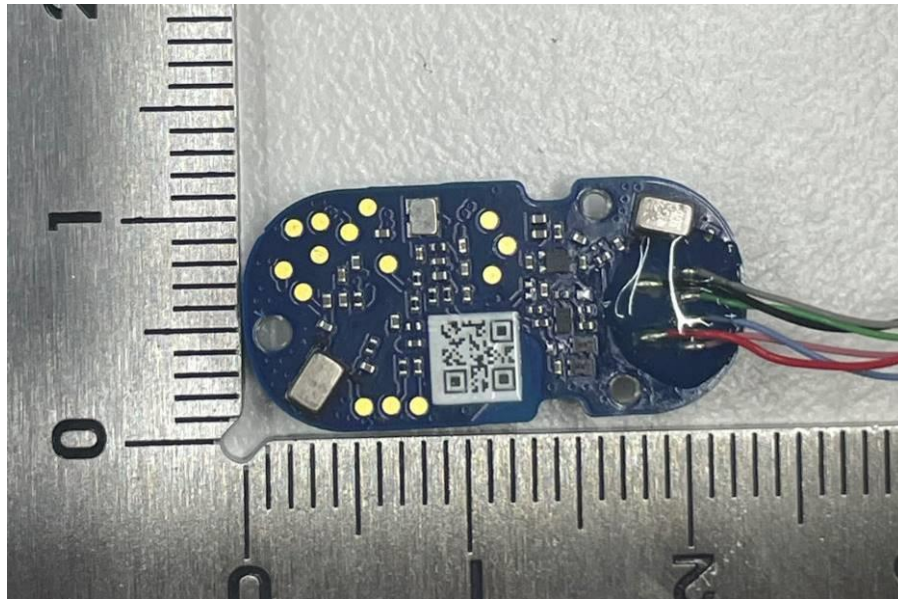
Figure 15: PCB view 1 of right earbud
