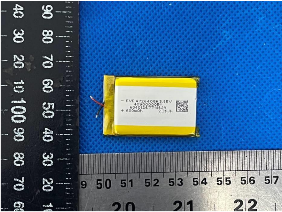
Figure 18: Battery view of charging case
